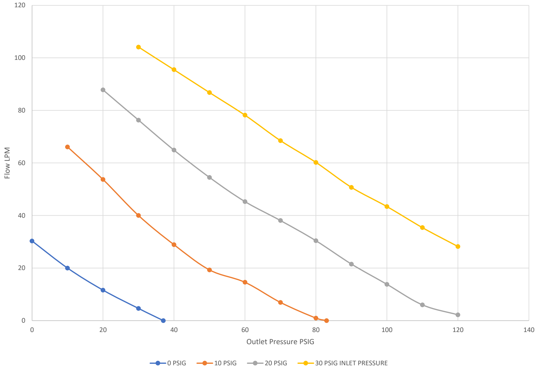
K181 Combination Curves
