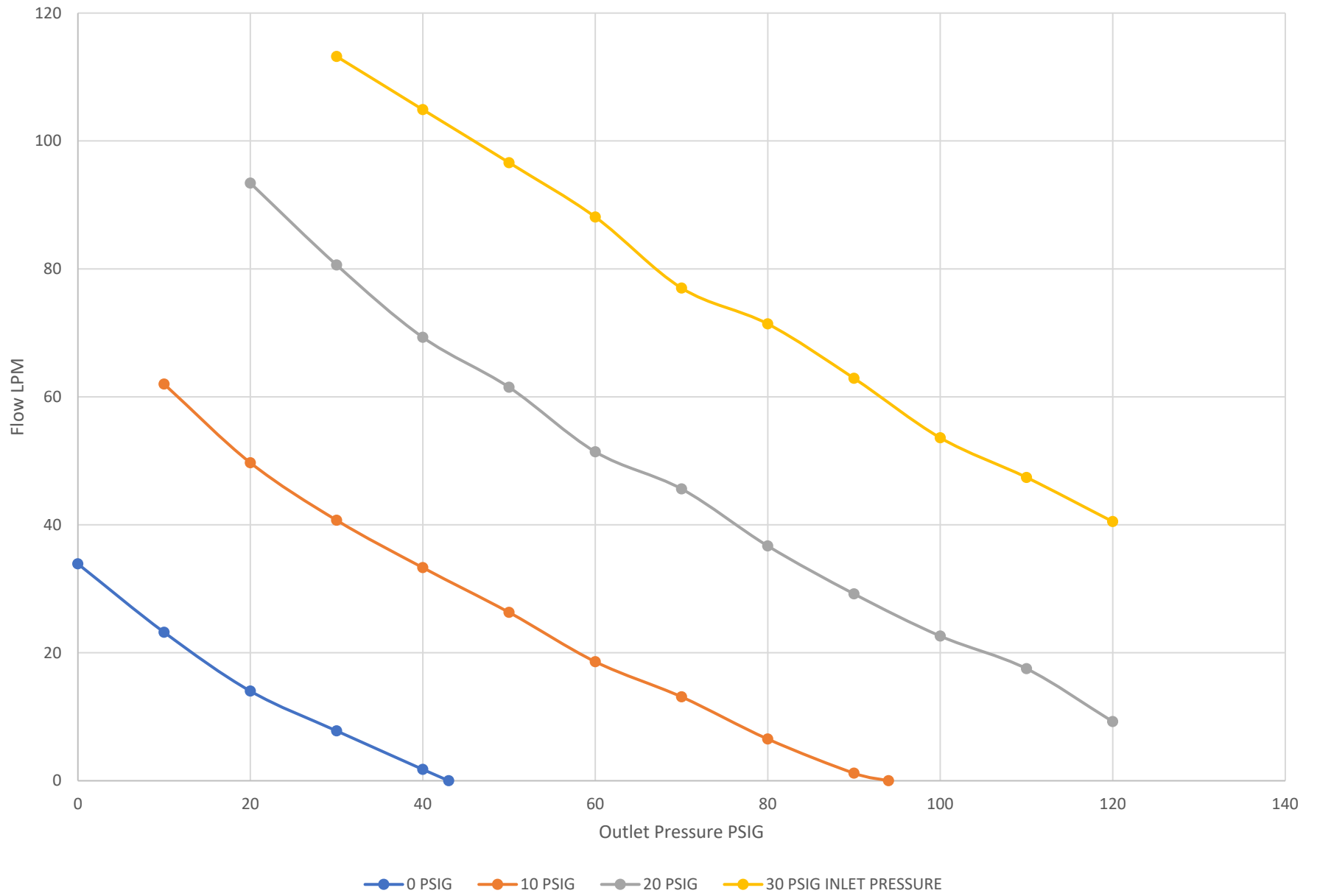
K201 Combination Curves
